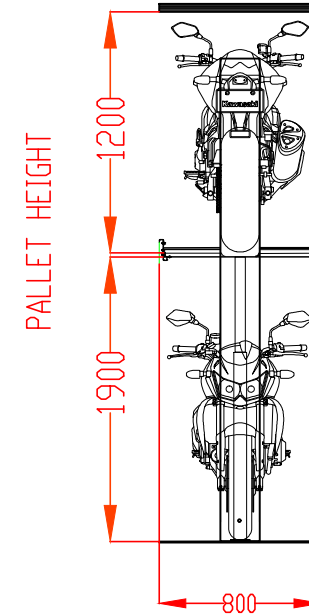
FRONT ELEVATION
