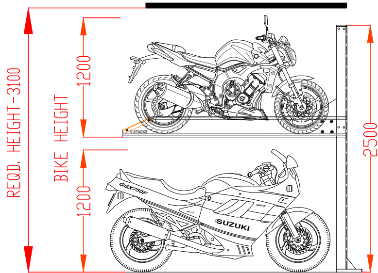
SIDE ELEVATION
