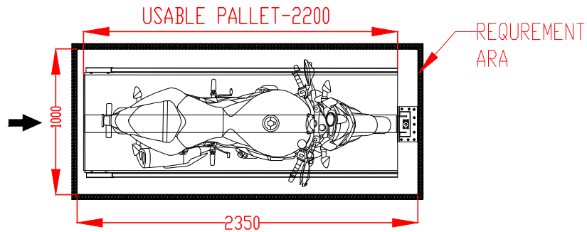
PALLET TOP VIEW
