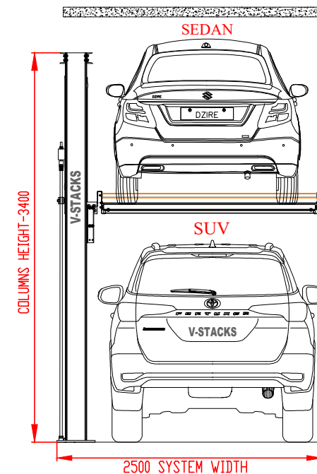
FRONT ELEVATION
