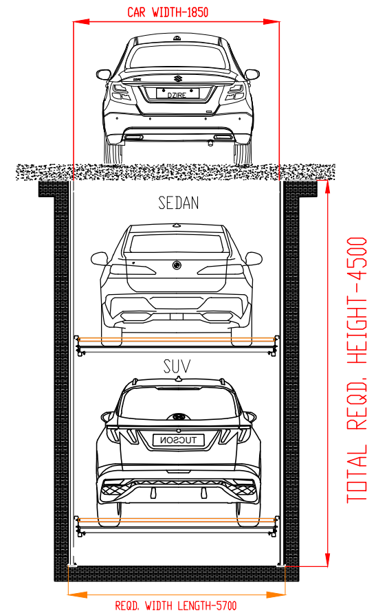
FRONT ELEVATION
